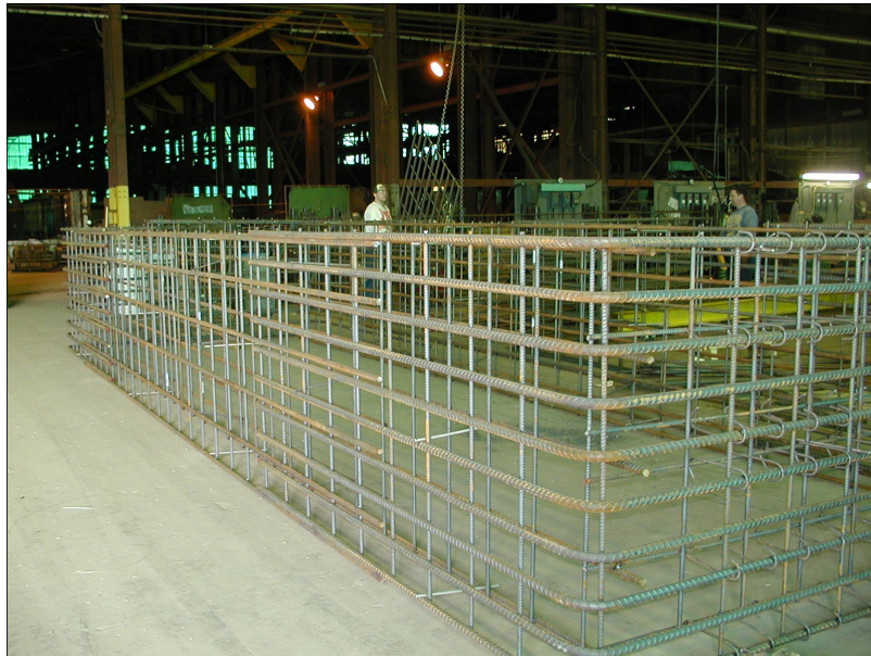
Pre-weld assembly, complete with stainless steel spacers, supplied to Hanson for insert into the Quick Span form, ready to receive concrete.
